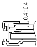
SECTION A-A SCALE 5/1
